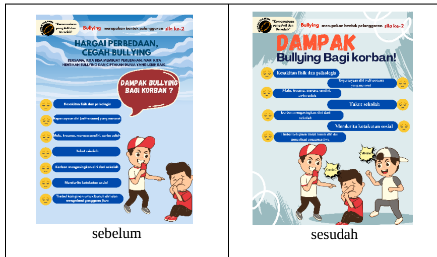
Gambar 1: Revisi media
