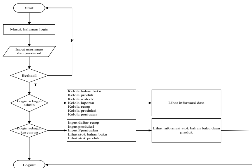
Gambar 3. Flowchart
