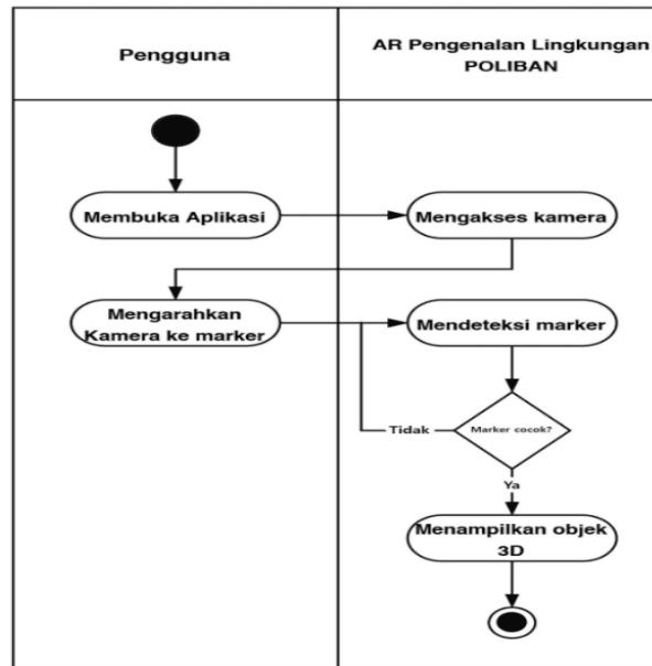
Figure 2. Activity Diagram
