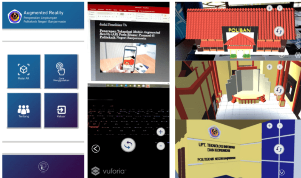
Figure 6. System Implementation
