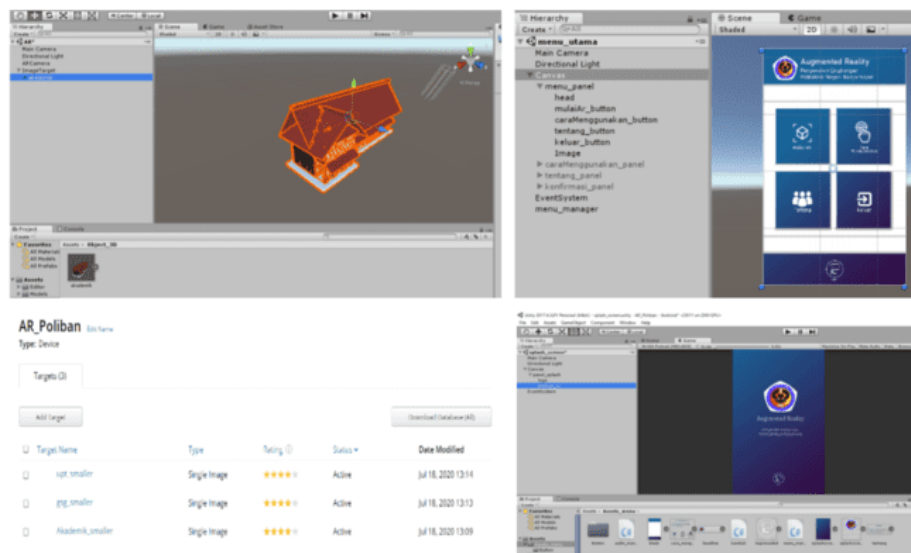
Figure 5. Coding Stages
