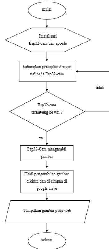
Gambar 13. Flowchart Proses Pengambilan Gambar Esp32-Cam
